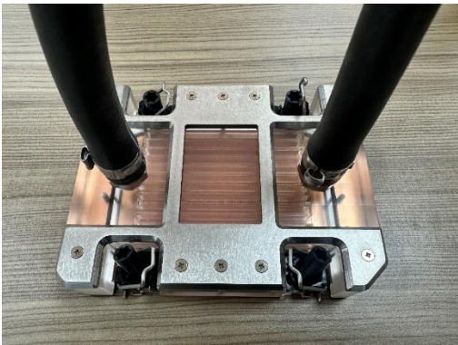
Intel LGA7529 1U Cold Plate
